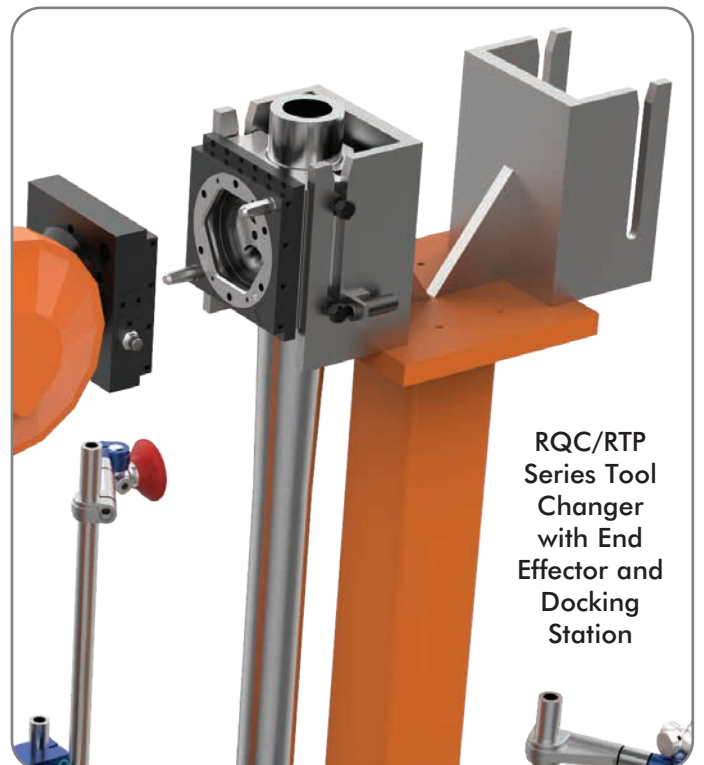
TP Series Tool Changer and Docking Station
